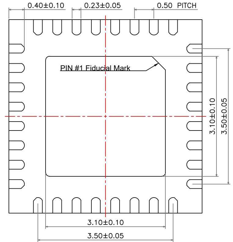
BOTTOM VIEW
